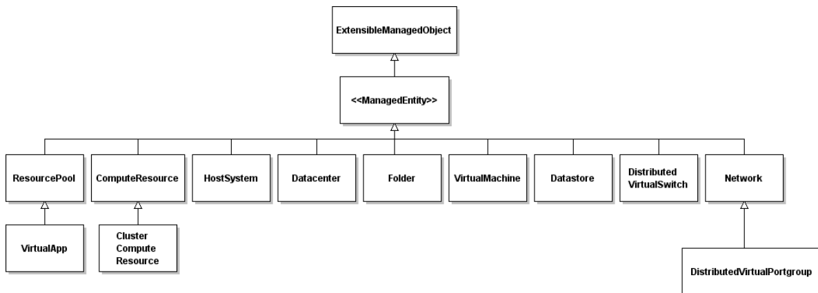
Figure 2-2. ExtensibleManagedObject Hierarchy
