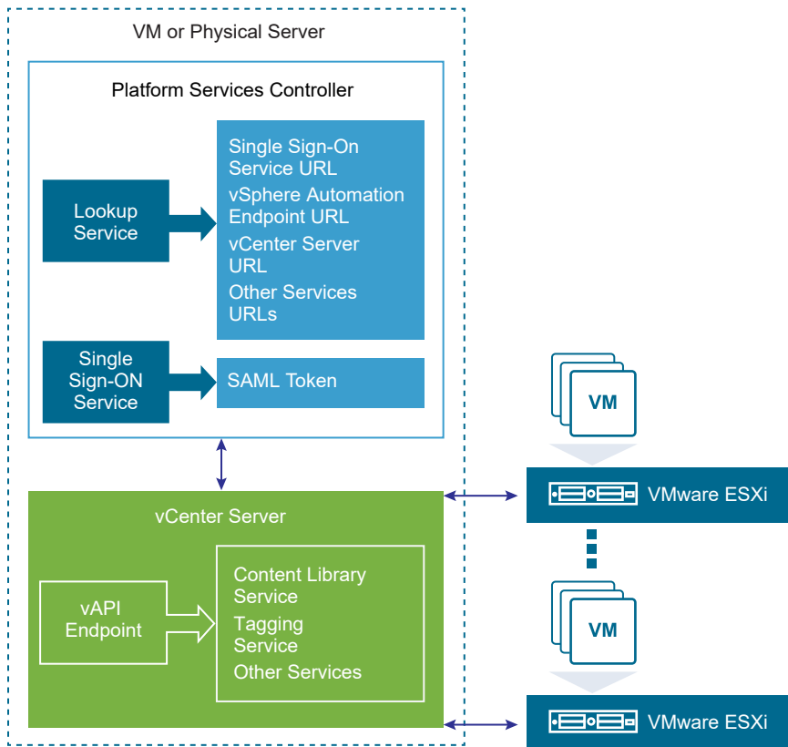
Figure 3-1. vCenter Server with Embedded Platform Services Controller
