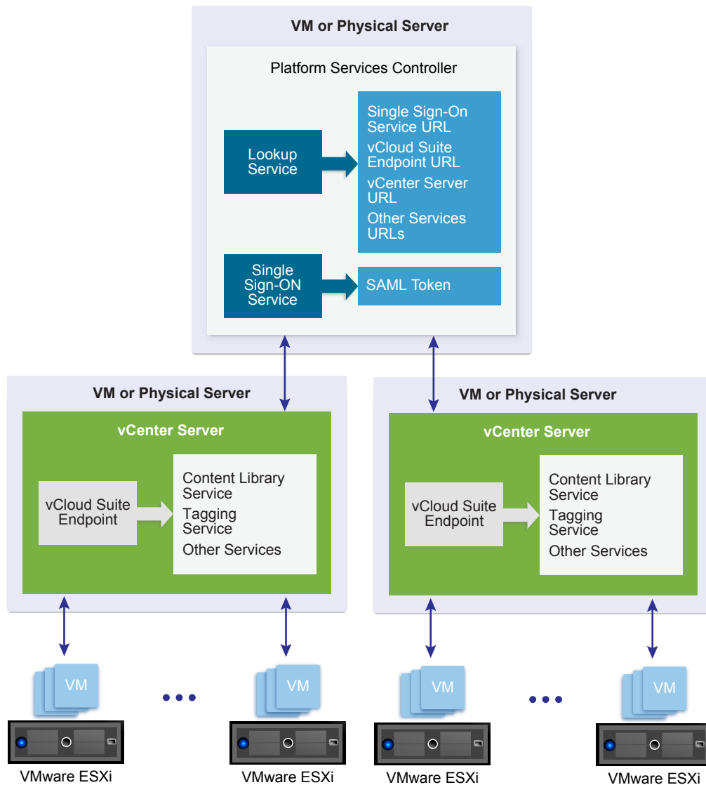
Figure 3-2. vCenter Server with External Platform Services Controller
