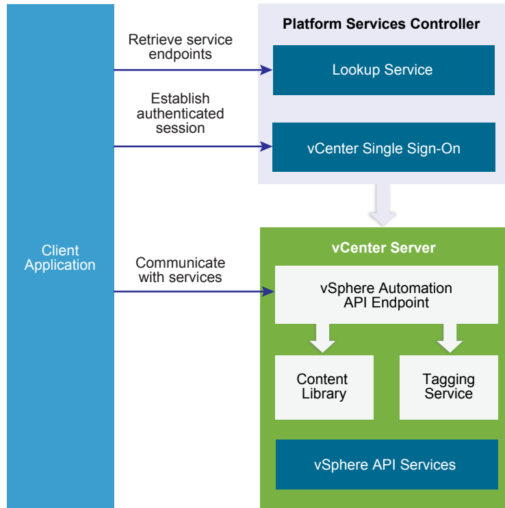
Figure 2-1. Communication Model of vSphere Automation API Client Applications
