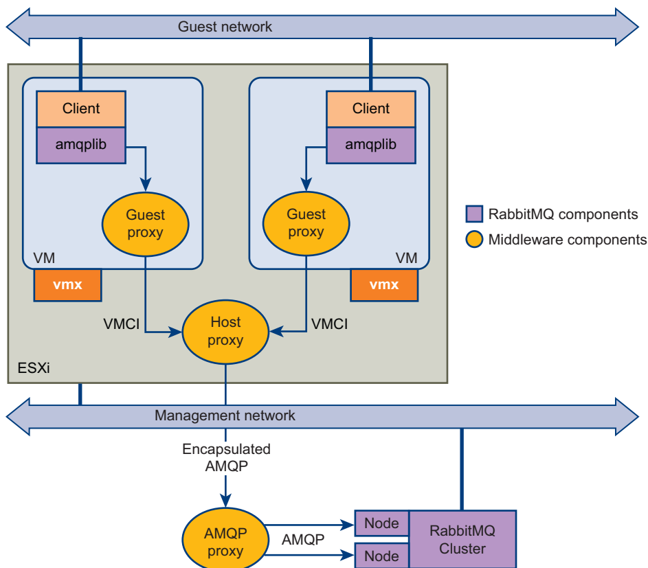
Figure 1-1. ESXi host with Stream VMCI Sockets and RabbitMQ
