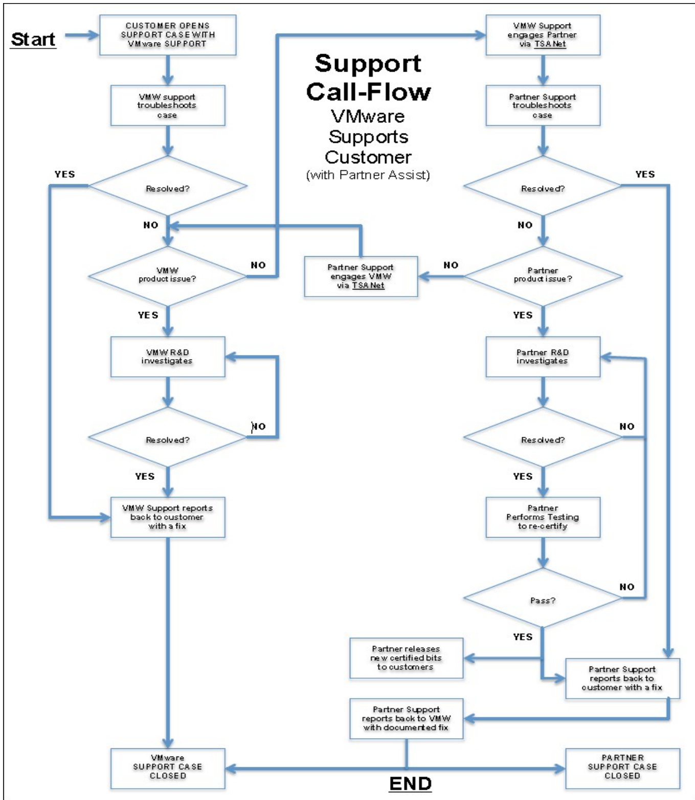
Figure 3: VMware Customer Contacts Support Flow.
